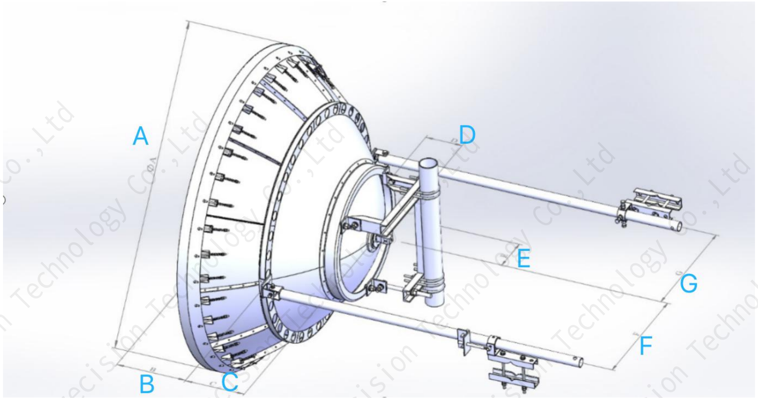
Dimensions in inches(mm)
